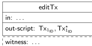
Figure 4: The special transaction editTx is broadcasted to the network to propose a redaction of transaction Tx 1 for the candidate transaction Tx 1 * .
