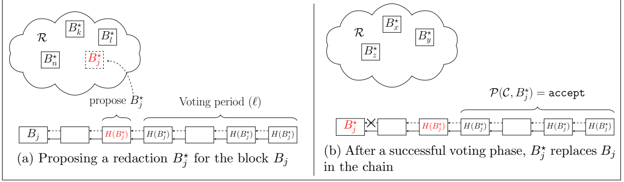
Figure 1: The candidate block pool \mathcal{R} stores the candidate blocks that are proposed and that can be endorsed in the voting phase. A block is linked to its predecessor by two links, the old link (solid arrow) and the new link (dashed arrow). In (a), a redact request B_j^* is proposed as a redaction for B_j and added to \mathcal{R} , then the hash of B_j^* is included in the chain to denote a new candidate redaction; its voting phase starts just after its proposal. In (b), the candidate block B_j^* has gathered enough votes and was approved by the redaction policy \mathcal{P} of the chain; B_j^* replaces B_j and the redacted chain is propagated. Note that new link from the block to the right of B_j^* is broken (marked by a cross), however the old link to B_j^* still holds. For simplicity, we consider the parameters k = 0 (persistence), \ell = 4 (voting period) and \rho \geq 3/4 (threshold for policy approval).
