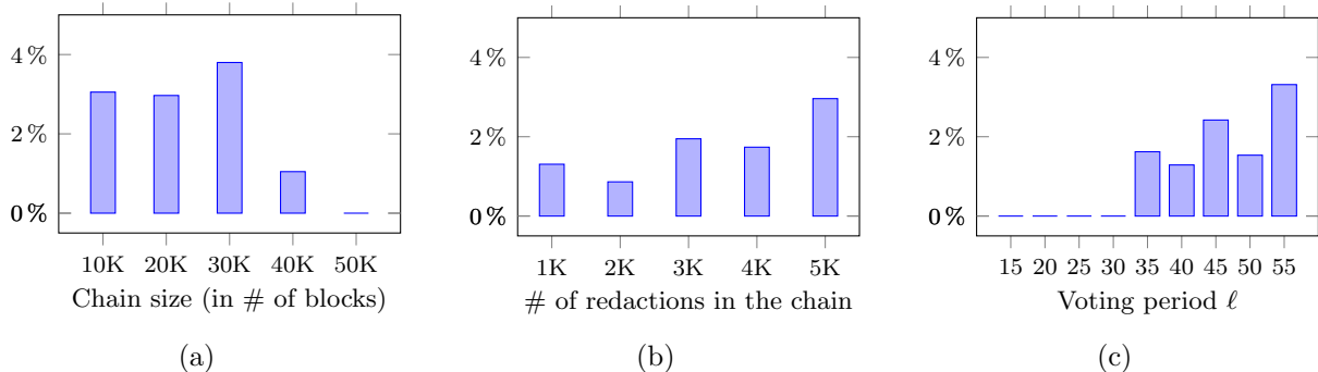
Figure 8: The graphs above show the overhead (in percentage) of our proof-of-concept implementation in each experiment performed. In (a) the graph shows the validation time overhead required to validate a redactable chain (with no redactions) compared to an immutable chain; in (b) the graph shows the validation time overhead required to validate a chain for an increasing number of redactions, compared to a redactable chain with no redactions, and finally in (c) the graph shows the validation time overhead required to validate a chain (with 1% of the blocks redacted) for increasing voting periods, compared to a chain (with 1% of the blocks redacted) on a fixed voting period of \ell = 5 .
